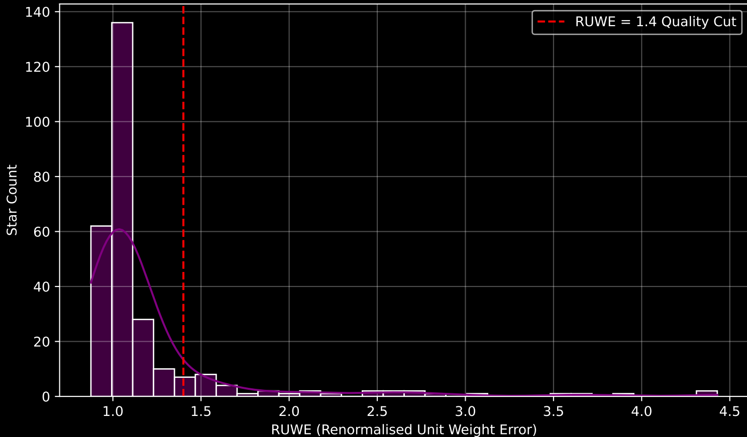
GALAH DR4 Field [1013] RUWE Distribution (n= 275)
