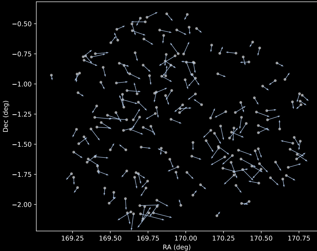
GALAH DR4 Cluster 1 Proper Motion Vectors (n=196)
