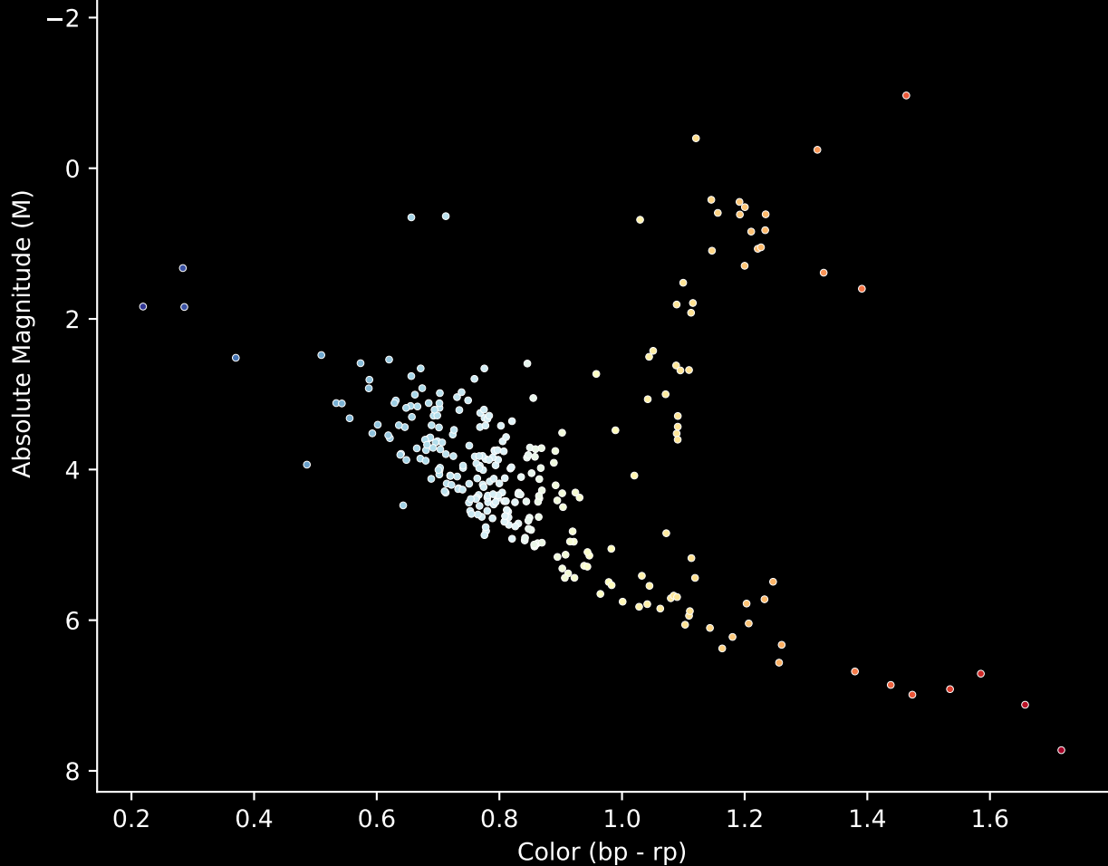
GALAH DR4 Field [1013] Stars (n= 285) Hertzsprung-Russel Diagram
