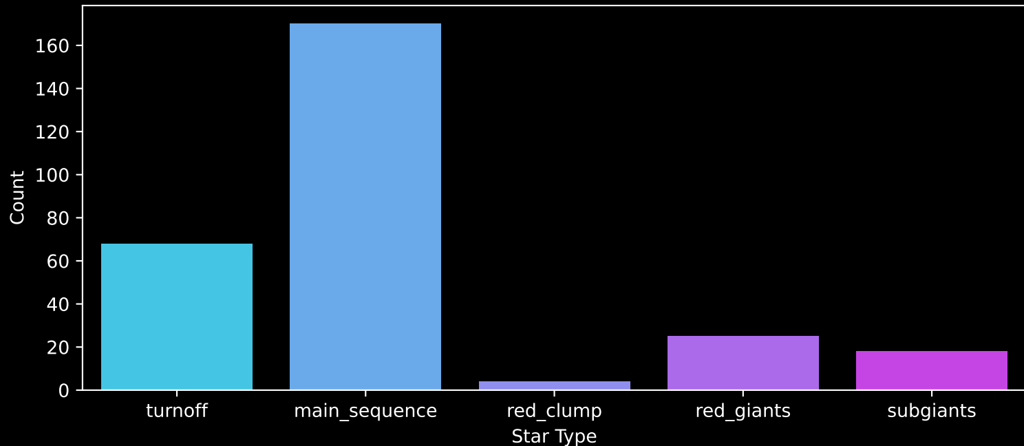
GALAH DR4 Field: [1013] Count plot of Star Type
